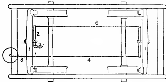
Fig. 1459. Plan. BRAKE FOR SHORT DROP-BOTTOM CAR.
